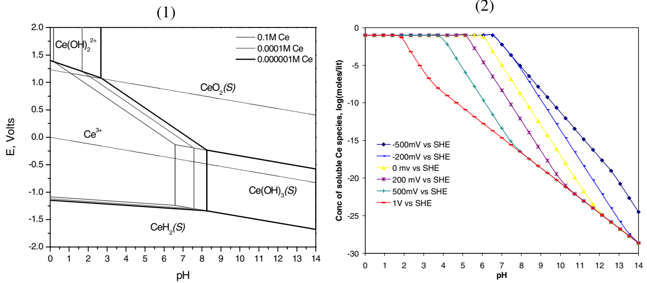
Figure 1: Potential – pH diagram of Cerium-Water system at different activities of soluble cerium species.
