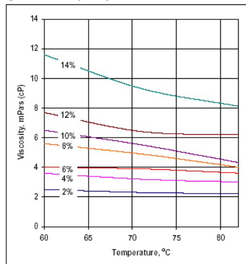
Figure 1. Viscosity/Temperature Curves for Elvanol ® 51-03
