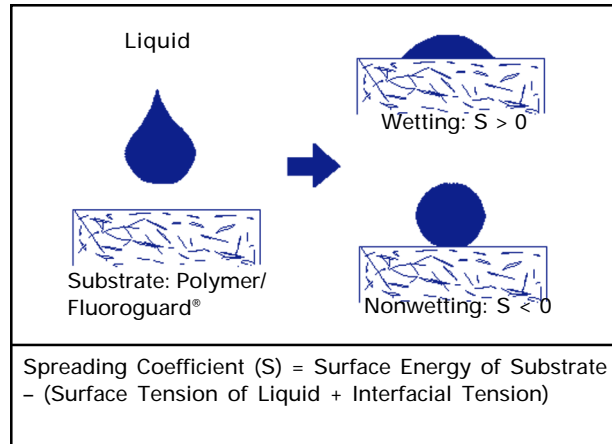
Figure 3. Schematic Diagram: Wetting and Nonwetting
