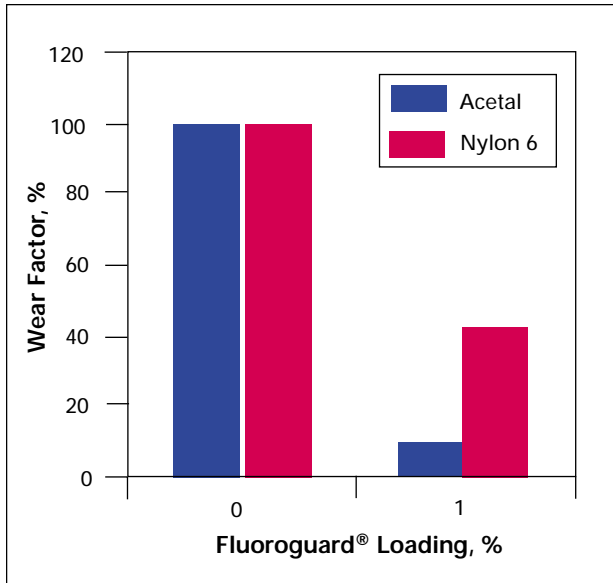
Figure 5. Polymer Wear per ASTM 3702 (vs. 1018C Steel at 40 psi, 50 ft/min)
