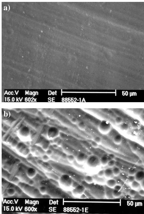
Figure 2. SEM Photographs of Molded Plaque Surface of a) TPU and b) TPU with 0.25% Fluoroguard®
