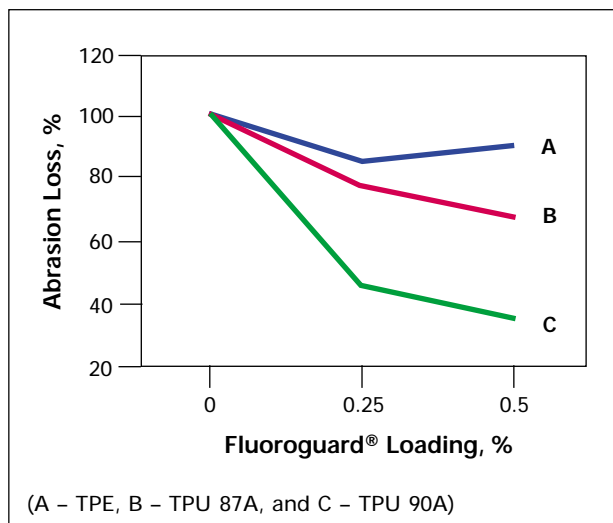
Figure 4. Abrasion Resistance of Thermoplastic Elastomers
