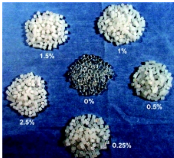
Figure 1. TPU with Different Fluoroguard® Loading Levels
