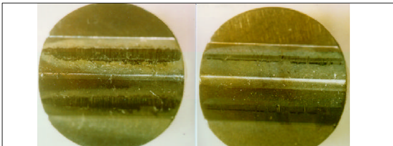
Pin and Vee Block Coupons (Large wear scar on left is from oil with no additives; the smaller scar on the right shows the effect of XP additives.)
