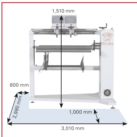
Technical Drawing
