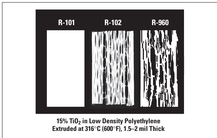
Figure 4. DuPont™ Titanium Dioxide Lacing Resistance
