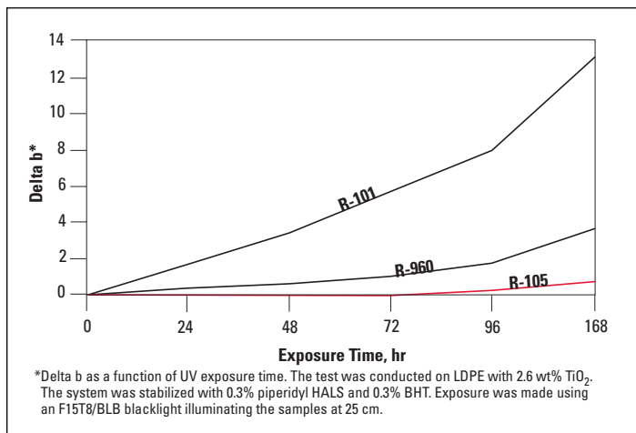
Figure 2. Discoloration Resistance
